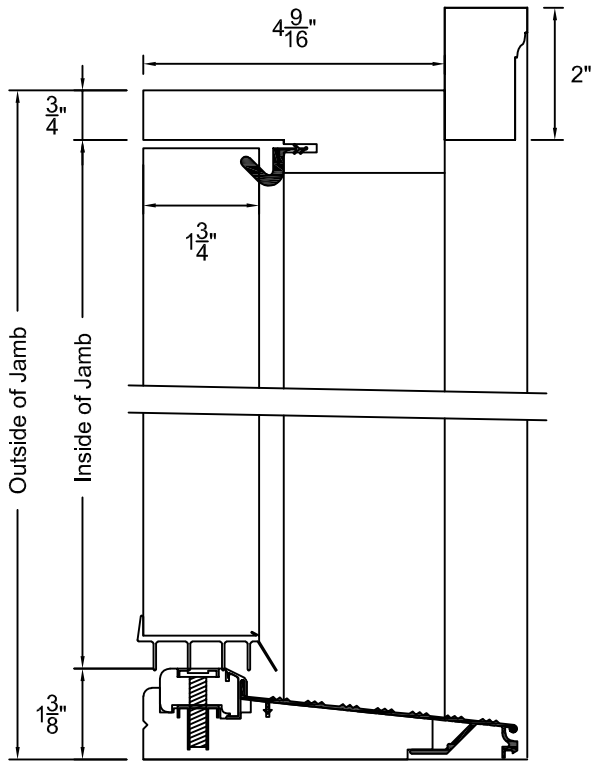
ADJUSTABLE SILL DETAIL
