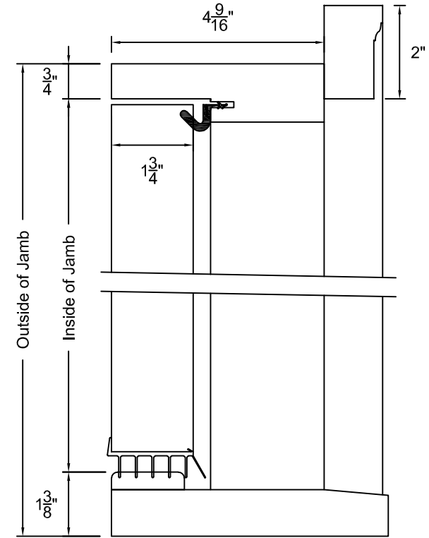
WOOD SILL DETAIL
