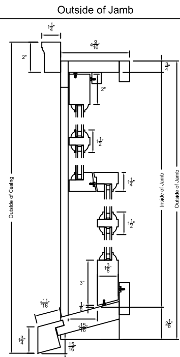
Double Hung
